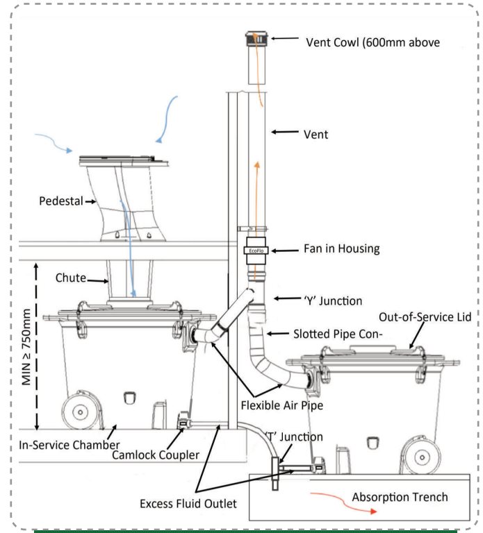
Side Profile of Classic 850
